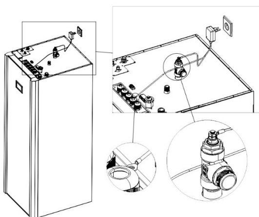
Figure 2 Anode on DHW outlet pipe (all other models)
