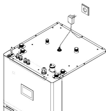
Figure 3 On newer models the anode can be installed directly on the 3/4" Female interface without using fittings. Except on UK units where the outgoing water pipe is used.
