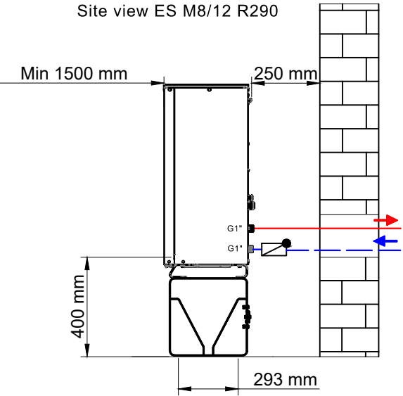
Site view ES M8/12 R290
