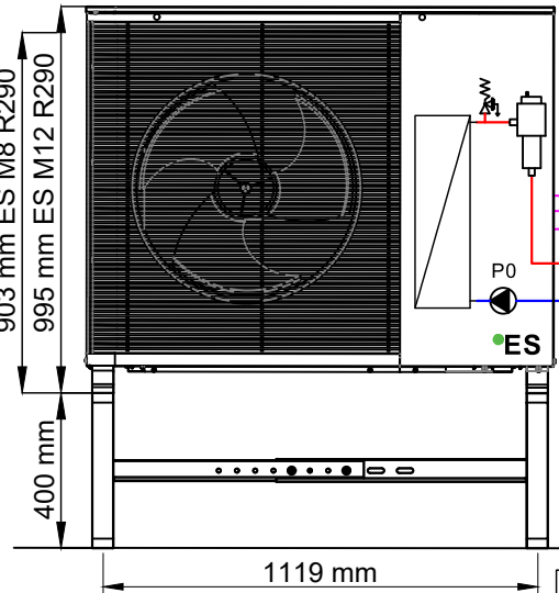
Front view ES M8/12 R290
