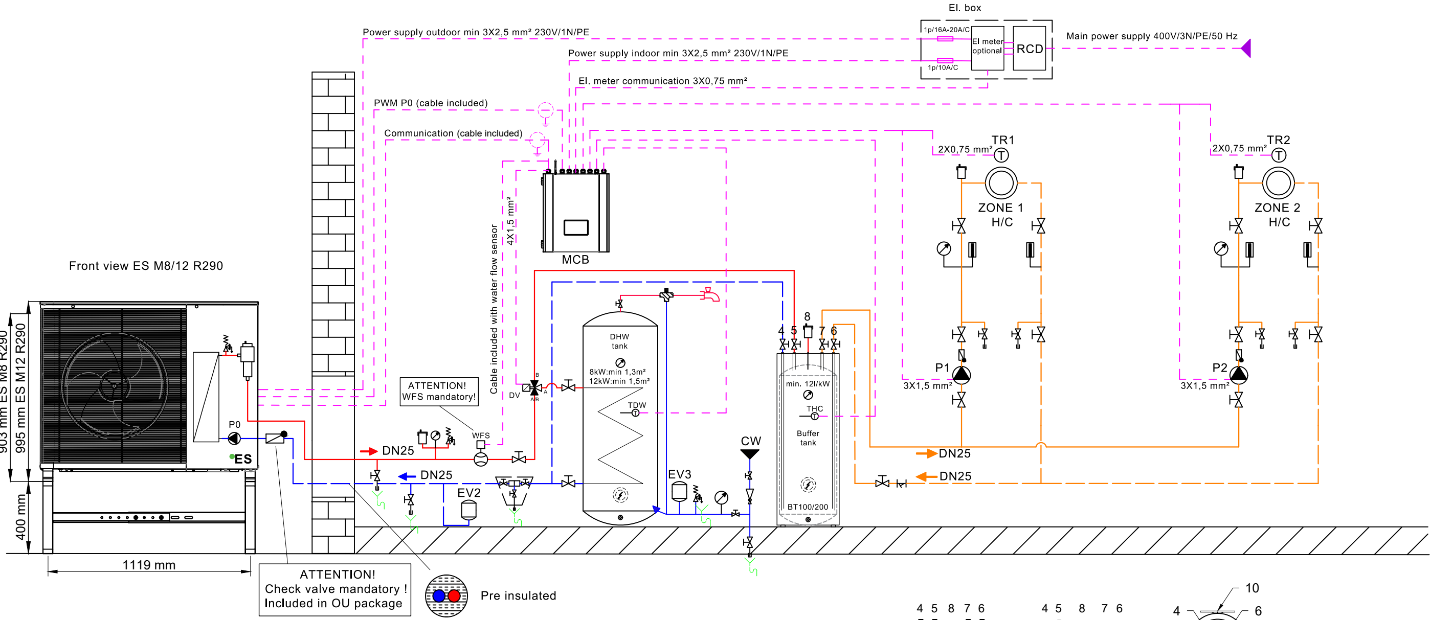
Site view ES M8/12 R290
